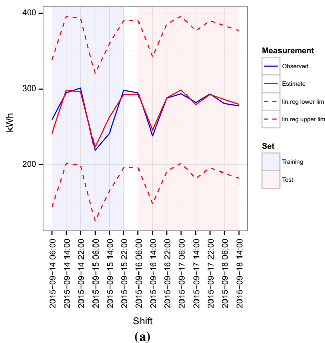
Fig. 3 Comparison of traditional linear regression and machine learning possible value ranges for the consumed energy estimate for a training and test set partition of the baseline data by 8-h shifts. a Consumed
